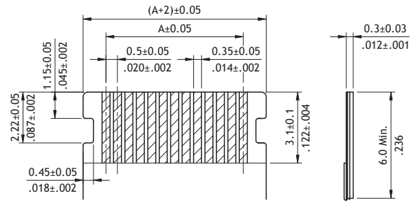
Accommodated FFC/FPC
