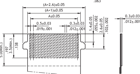
Accommodated FFC/FPC
