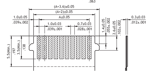
Accommodated FFC/FPC
