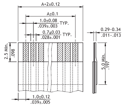
Accommodated FFC/FPC
