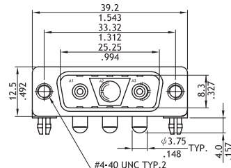
3W3C (Plug Connector)
