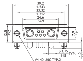
C7W2 (Receptacle Connector)
