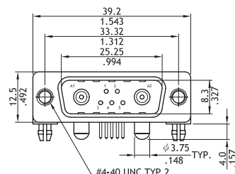
C7W2 (Plug Connector)
