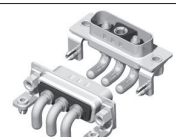
3W3C (Receptacle Connector)
