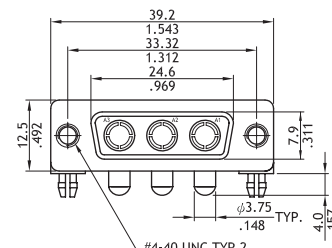
C3W3 (Receptacle Connector)
