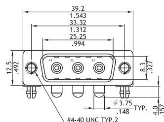
C3W3 (Plug Connector)
