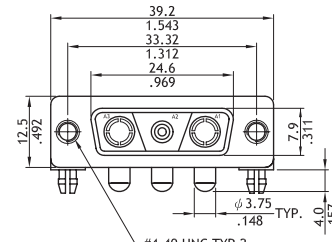
3W3C (Receptacle Connector)
