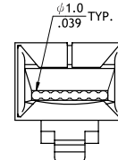
Flat-oval Cable
