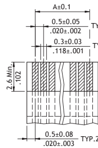
Accommodated FFC
