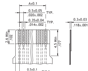
Accommodated FPC
