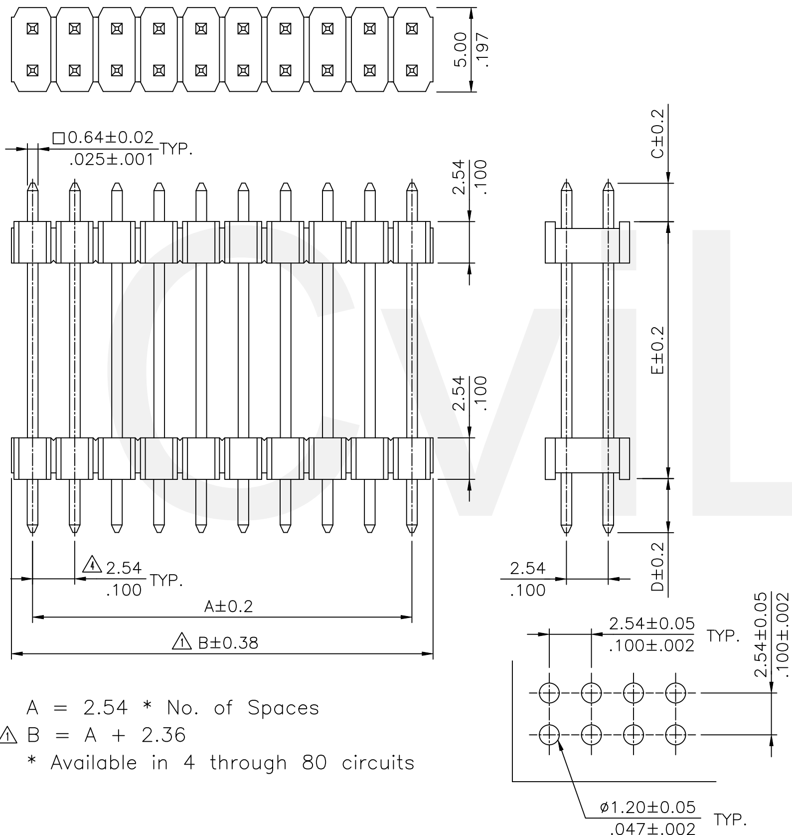
Recommended P.C. Board Layout
