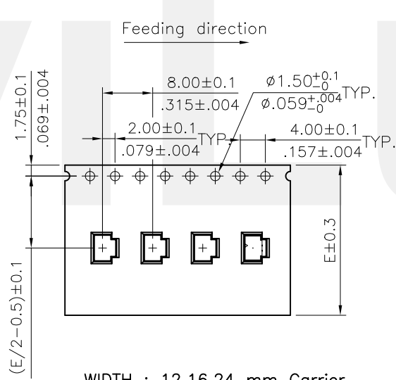
WIDTH : 12,16,24 mm Carrier
