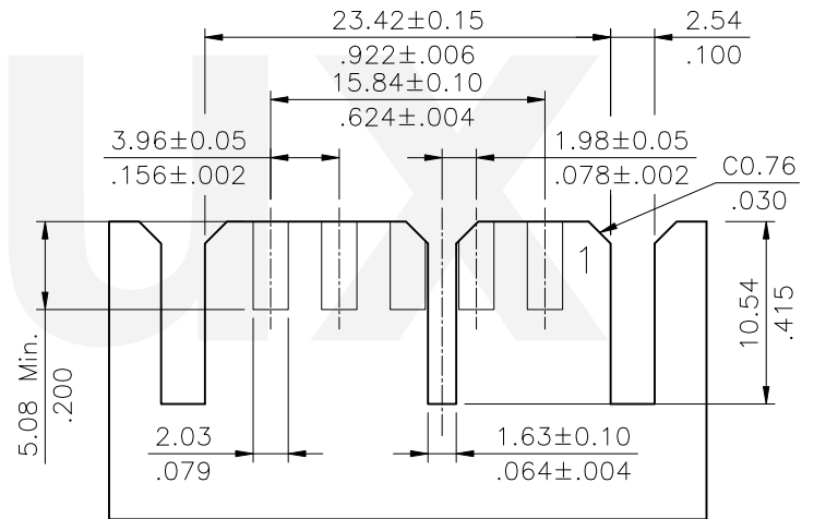
Generic PCB Layout PCB Thickness: 1.57mm
