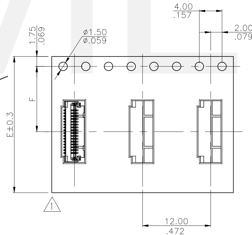
WIDTH : 16.24 mm Carrier (SCALE 1:4)
