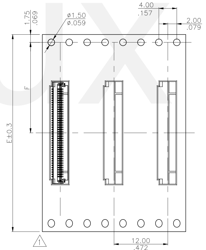
WIDTH : 32 mm Carrier (SCALE 1:4)
