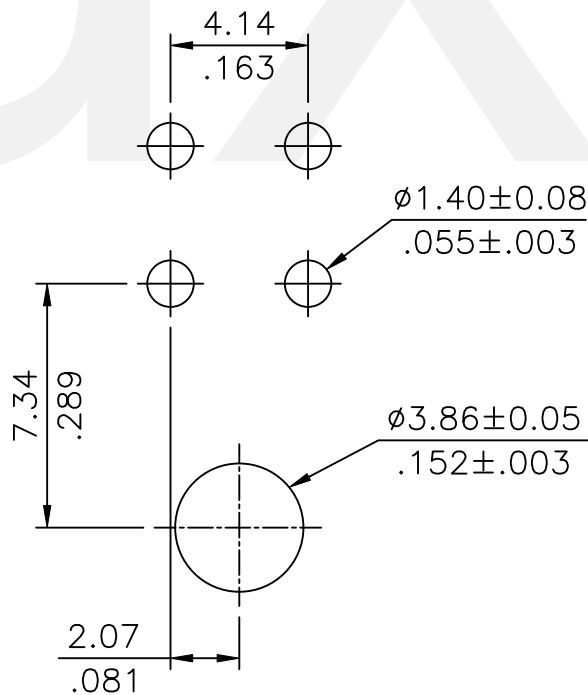
Recommended P.C. Board Layout
